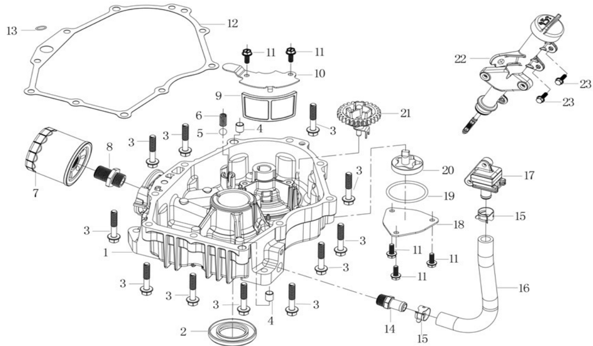
曲轴箱盖 ( CRANKCASE COVER )
